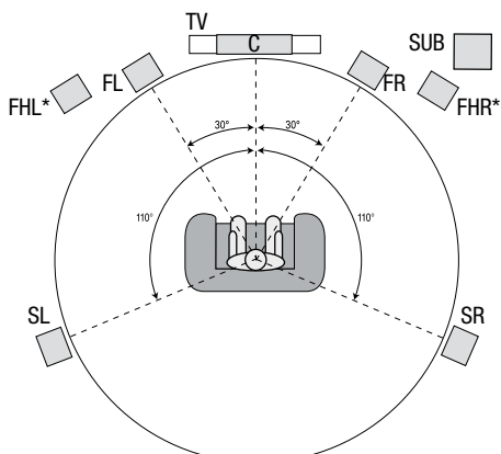
Speaker Positioning for 7.1-Channel Systems
